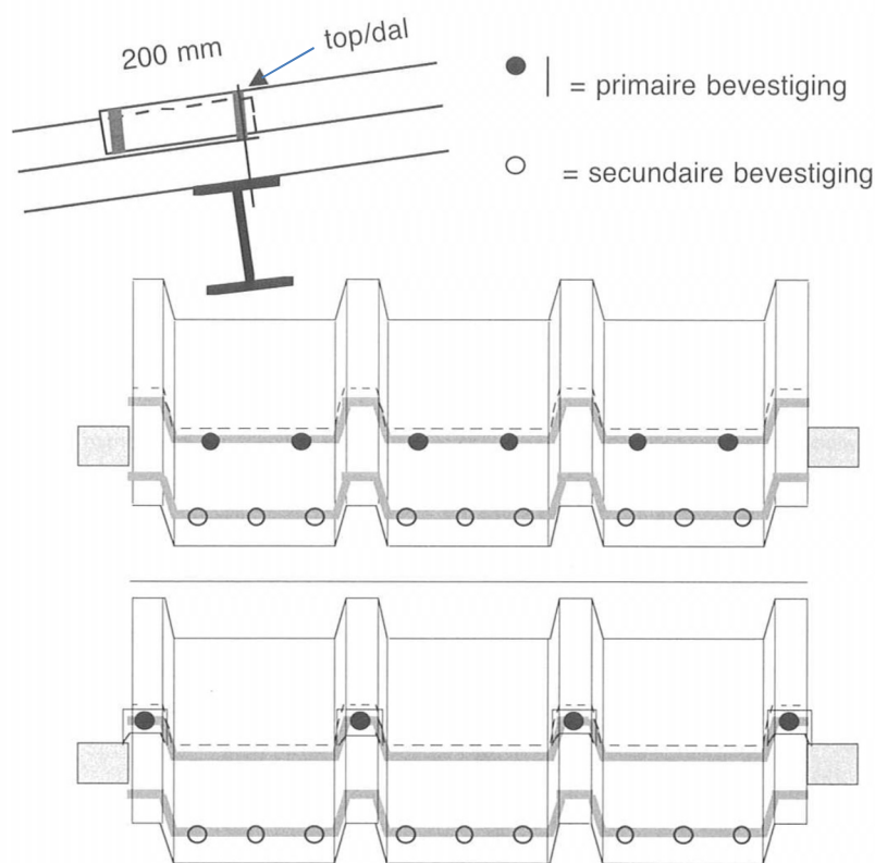
> 7°: overlap 200 mm en 2 afdichtingen
